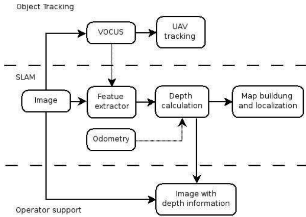
Figure 7. Schematic overview of the vision systems.
