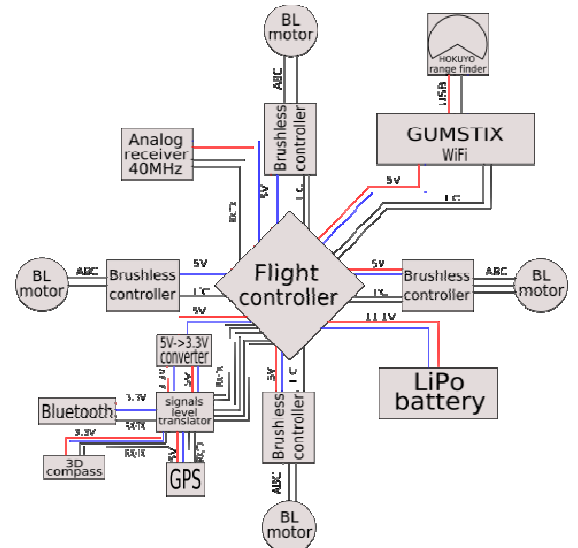
Figure 9. The quadrotor's functional diagram with distributed
