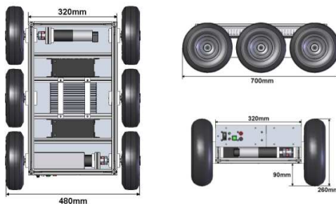
Figure 3. Engineering drawing of the VolksBot RT6 chassis. RT6 is a six-wheeled robot platform with rough terrain capabilities. The left sketch shows top view, upper right shows lateral view and lower right shows front view.
