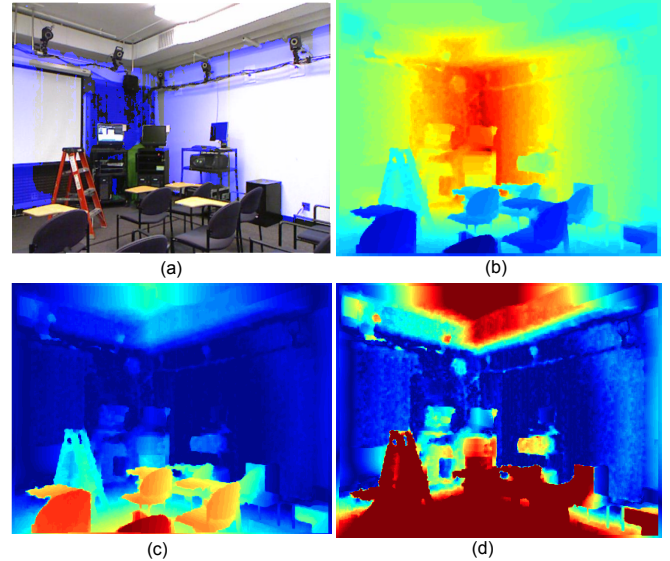
Fig. 1. Illustrating the distance-from-wall feature. (a) Color image with its blue channel replaced with the binary mask based on the bounding hull heuristic from [7]. The walls are detected from the bounding hull region. (b) Depth image, (c) and (d) show the minimum distance of each point in the scene from the walls before and after thresholding, respectively.
