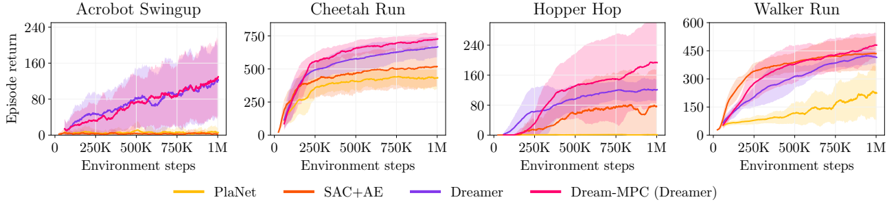
Figure 13. Learning curves for four tasks from the DeepMind Control Suite. The line represents the mean episodic return and the shaded area the 95% confidence interval across 3 seeds.
