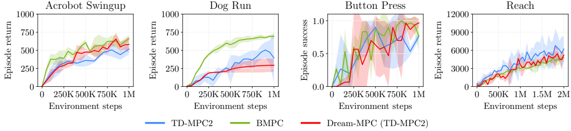
Figure 4. Learning curves for four tasks from the DeepMind Control Suite, Meta-World and HumanoidBench. The line represents the mean episodic return and the shaded area the 95% confidence interval across 3 seeds.
