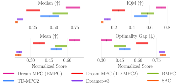
Figure 1. Aggregate performance metrics. Optimality gap, interquartile median (IQM), mean and median normalized scores with 95% confidence intervals of different methods. Notably, Dream-MPC with a strong policy achieves the best results.
