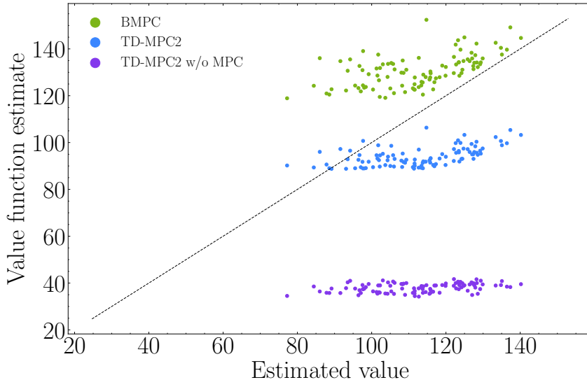
Figure 19. Value estimation comparison for BMPC policy on Dog Run.
