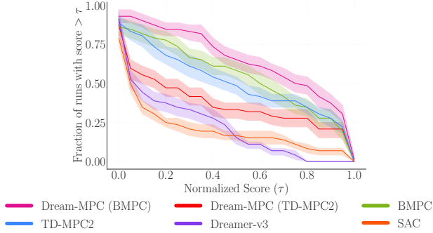
Figure 3. Performance profiles. Score distributions across all tasks, which provides insights into the variance of the performance. Detailed results are included in Tabs. 11 to 13.
