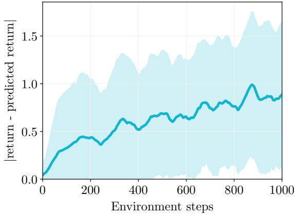
(a) Mean difference between actual and predicted returns and standard deviation for three different seeds and ten test episodes per seed.
