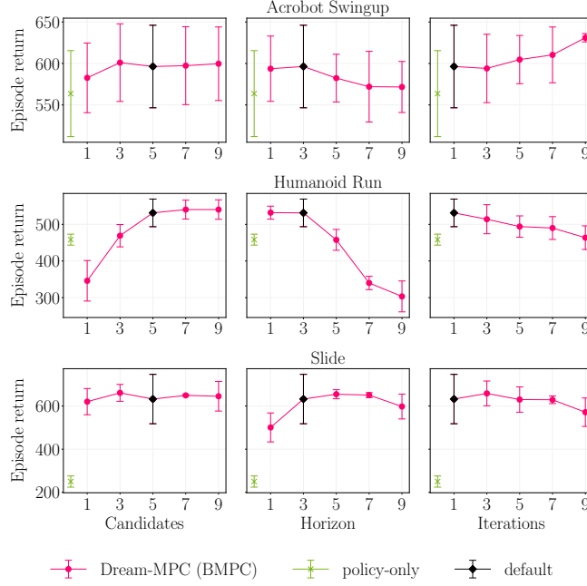
Figure 12. Parameter sweep. Performance of trained BMPC agents with Dream-MPC at test time when varying the number of candidates, horizon and number of optimization iterations. When varying one hyperparameter, the others are fixed to their default value. We also include the performance of the learned policy \pi_\theta and the default values of one iteration, a horizon of three and five candidate trajectories.
