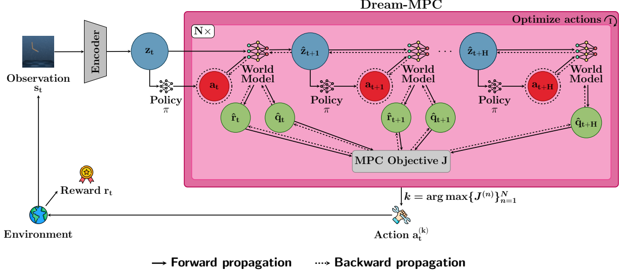
Figure 2. Overview of the proposed approach. Dream-MPC optimizes action sequences rolled out from a policy network \pi in latent space z with gradient-based MPC. N candidate trajectories are sampled from the policy prior and optimized for I iterations using gradient ascent to maximize the objective J . The first action from the candidate trajectory with the highest value of J is applied to the environment, and the procedure is repeated for the next time step. The policy network and world model are shared across candidates and time steps.
