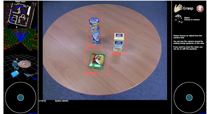
Fig. 1. Skill and body-level GUI with a view selection column on the left, a main view in the center, a configuration column on the right, and a log message window on the bottom center. Motion is controlled directly with two joystick control UIs.
