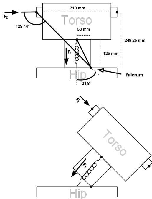
Fig. 8. Analysis of the effect of the ground reaction force. The cylinder creates a fulcrum on the hip frame and the torso works as a lever against the spring. At the shoulder a joint a force of 12.8 N ( F_2 ) is needed to expand the spring pulling at the center of the torso with an initial force of 64 N ( F_1 )
