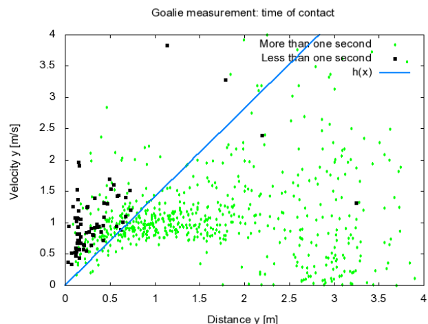
Fig. 2. Classification of ball observations into two categories: reaching the goal in less than one second or more than one second. The linear function h(x) separates the data. The goalie jumps only if the ball is estimated to reach the goal in less than one second.
