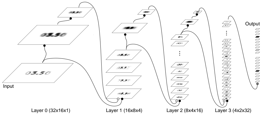
Figure 3: Network architecture for recognition of entire meter value blocks.
