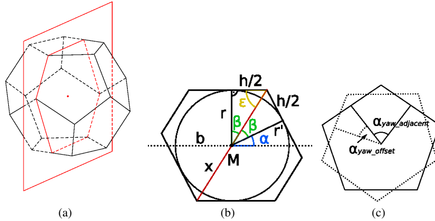
Fig. 8. Geometry of a penta-dodecahedron. (a) Slice plane through the dodecahedron. [18] (b) Dodecahedron with angles \alpha , \beta and \varepsilon . x denotes the axis of symmetry. (c) Yaw angles seen from top perspective.
