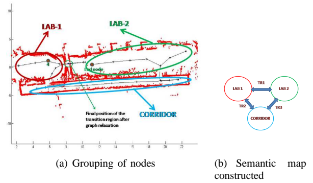
Fig. 4. Semantic Mapping
