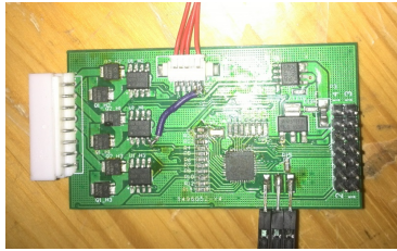
Fig. 5. BLDC Driver Demo Board
