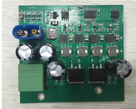
Fig. 7. Demo Board of New Power Supply Subsystem
