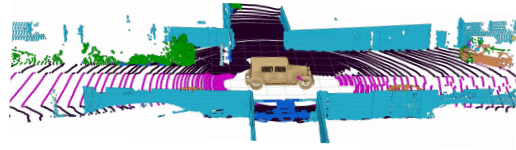
Figure 8: Point cloud segmented by LatticeNet (Rosu et al., 2020) and visualized with the colormap of SemanticKITTI (Behley et al., 2019).
