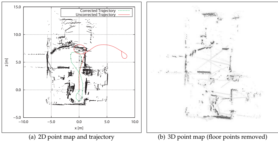
Fig. 10. Shown here are a two-dimensional sparse point map (a) as well as three-dimensional sparse point map (b) of an example scenario. Measurements corresponding to flat floor have been removed.
