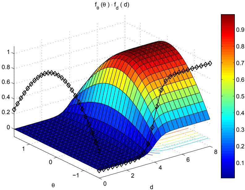
Fig. 7. Composed weighting function f_{\theta}(s_i^{\theta}) \cdot f_d(s_i^d) to determine the freespace orientation in a laser scan or obstacle map S .
