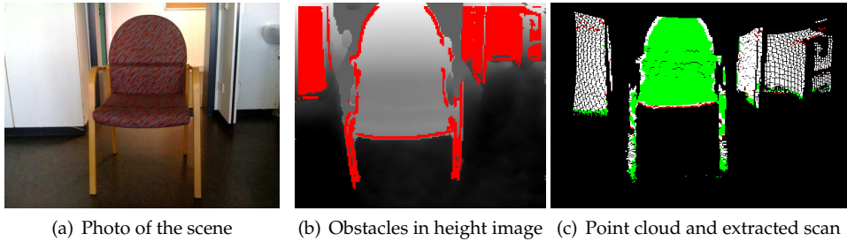
Fig. 14. Detecting obstacles in the filtered height image of an example scenario (a). Those obstacles in the height image (b) that form the closest obstacles in the respective direction and are comprised in the virtual scan are marked red. Obstacle points not contributing to the virtual scan are marked white.
