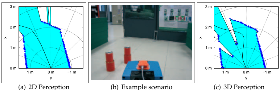
Fig. 8. Behavior-based collision avoidance in an example scenario by means of 2D perception (2D laser range finder in a fixed horizontal position) and continuous 3D perception together with the concept of obstacles maps. The small test objects are successfully avoided by the robot when using 3D perception. A video showing the robot perform in a similar experiment is available under http://www.b-it-bots.de/media .
