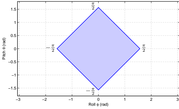
Fig. 2. Valid domain of fused pitch and roll, as per the sine sum criterion.
