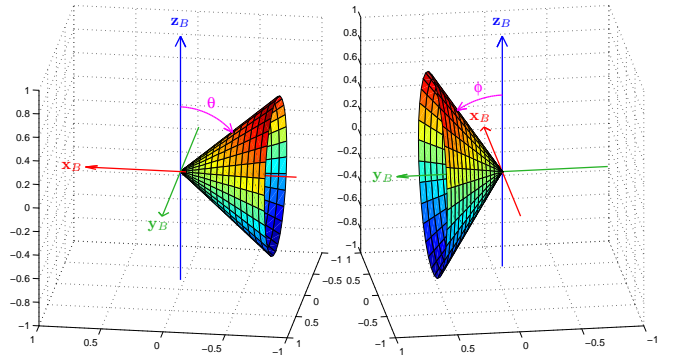
Fig. 3. Cones of constant fused pitch \theta (left) and fused roll \phi (right).
