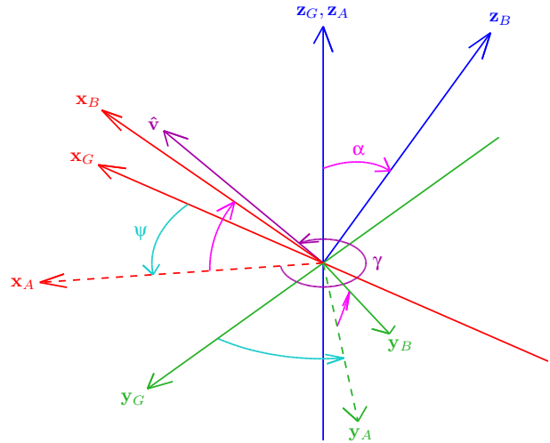
Fig. 1. Definition of the tilt rotation and tilt angles parameters (\psi, \gamma, \alpha) .
